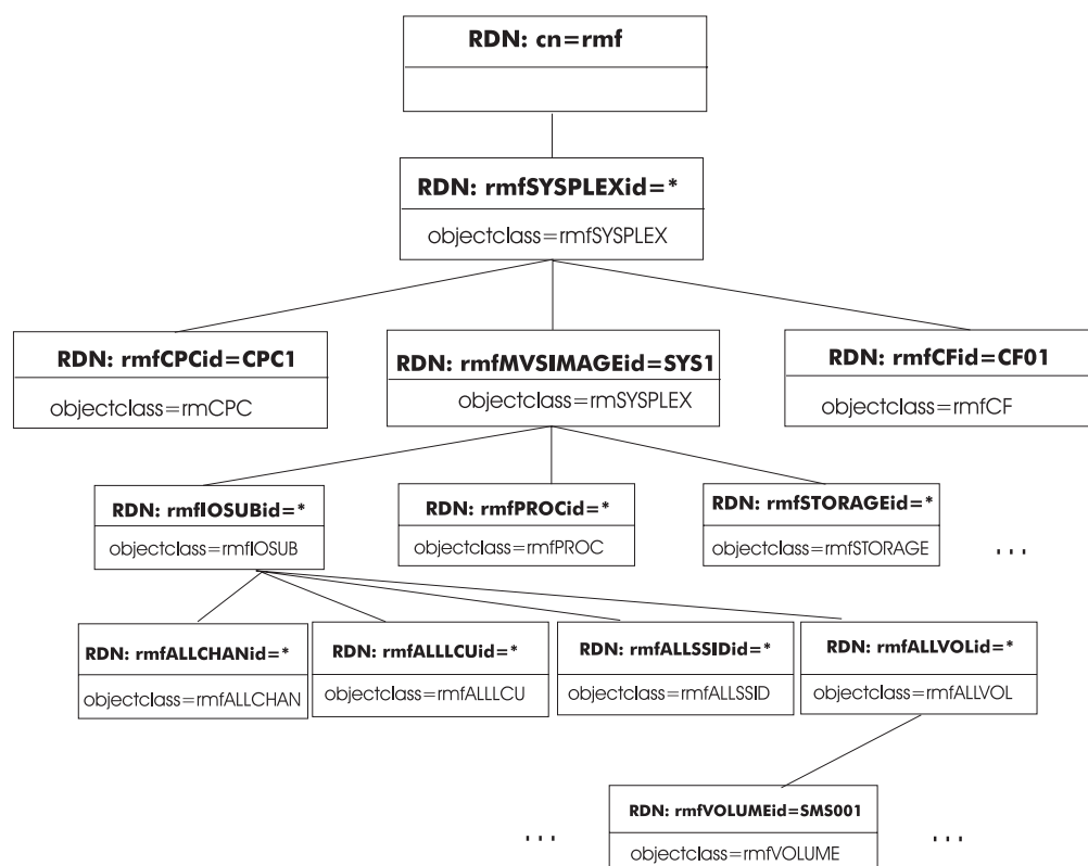
Figure 8. Sample DIT Portion of the RMF LDAP Performance Data
