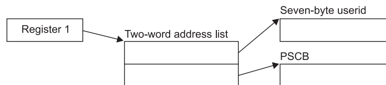
Figure 48. ERB3SOCK Input Parameter Structure
