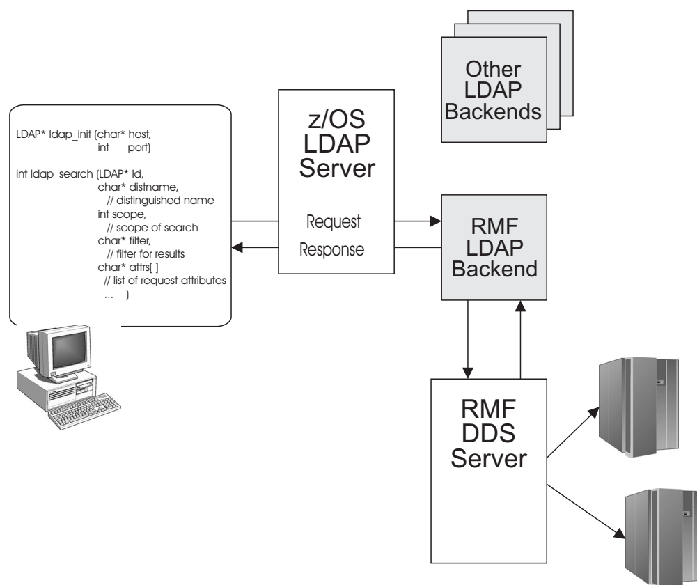
Figure 9. Accessing Performance Data from LDAP
