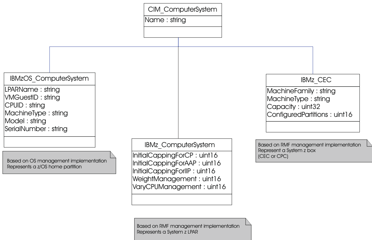
Figure 7. z/OS resource classes implemented by RMF. Simplified subset of LPAR- and CEC-related resource classes
