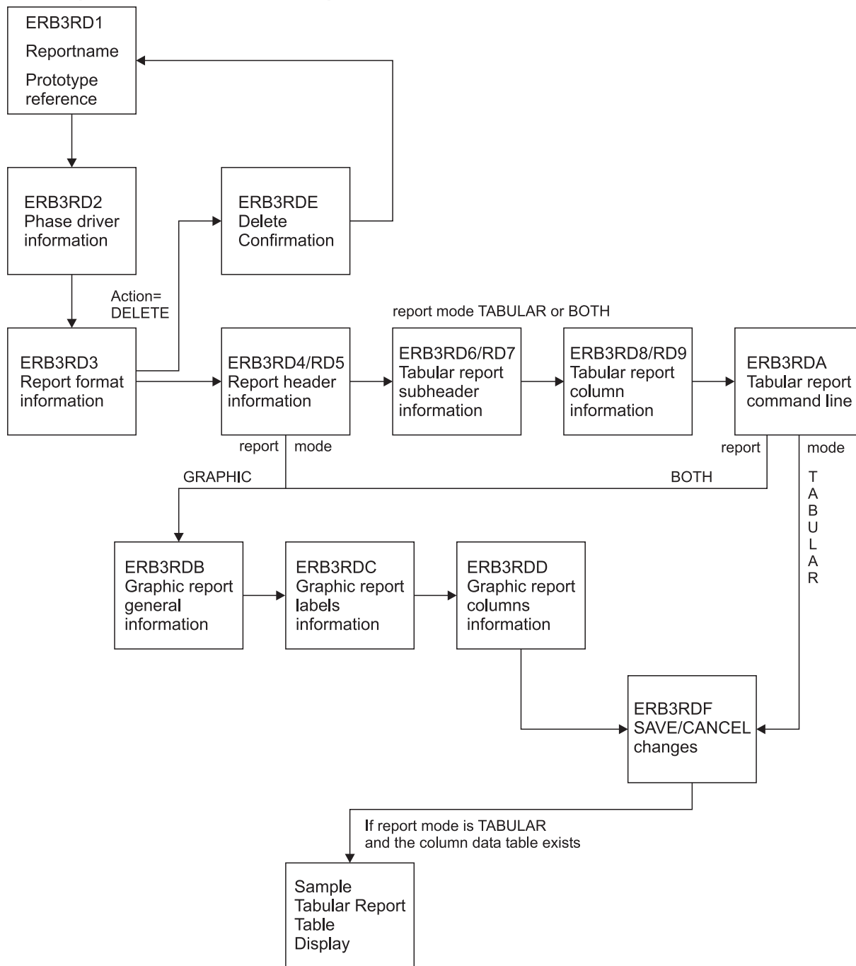
Figure 27. Panel Sequence for the Report Definition Utility
